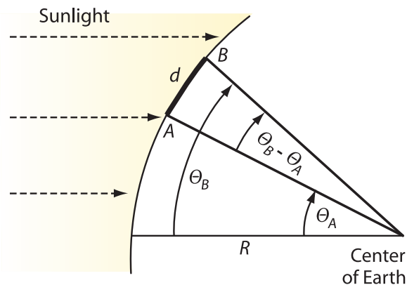
Figure 5: The geometry for measuring the radius of Earth using the data of two collaborating schools separated by a north-south distance. Each will measure the angle of the sun, \theta_A at one location and \theta_B at the other, at local noon.
